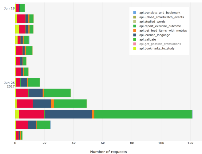
Fig. 2. The number of requests per endpoint per day view shows the overall utilization of the monitored application
